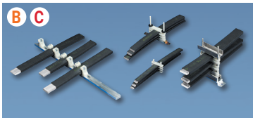
nVent ERIFLEX Flexibar Supports
