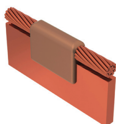
LW Ease of Use: PREFERRED Mold Split: -
