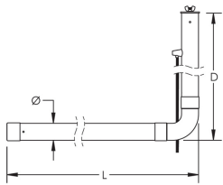
Horizontal with Pigtail Down
