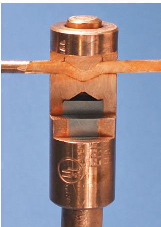
Hammerlock cutaway.
